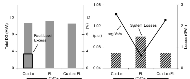
Fig 6. Maximum DG capacity (left) and network characteristics (right) for active network schemes: co-ordinated voltage control (CVC), wind energy curtailment (Cu), loss limits (Lo), and fault levels (FL).
