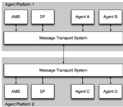
Fig. 1. FIPA Agent Management Reference model.
