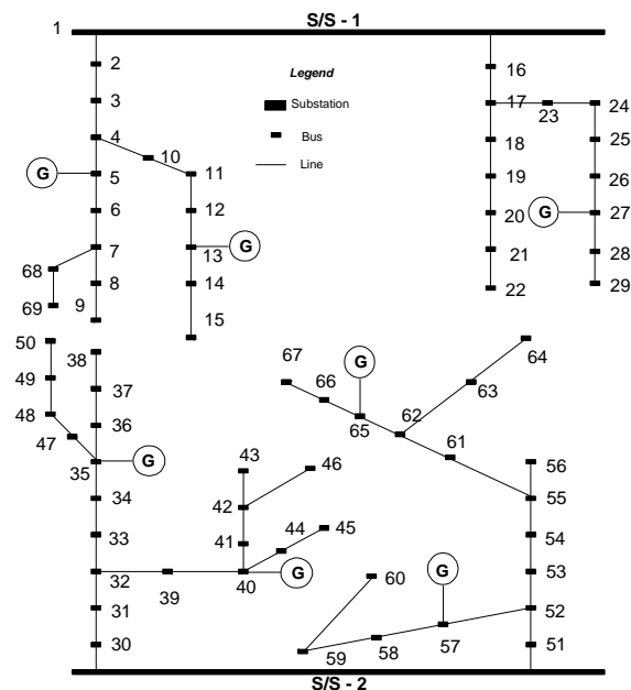
Fig. 1. 69-bus Network with DG unit locations
