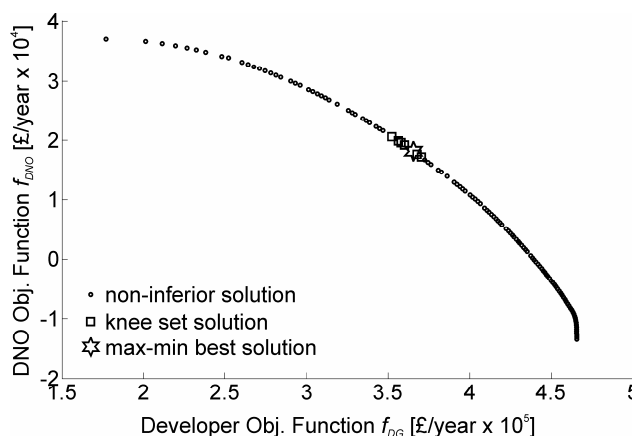
Fig. 2. Pareto solutions
